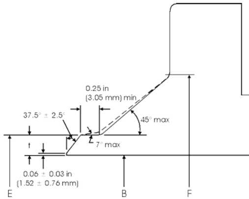
ASME/ANSI B16.5 (NPS 1/2 to 24) Weld Neck Flange Bevel (with no backing ring) for Wall Thicknesses (t) from 0.19 to 0.88 in (4.83 to 22.35 mm).
