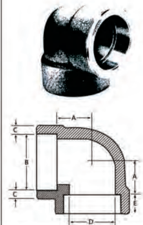
90° elbow
