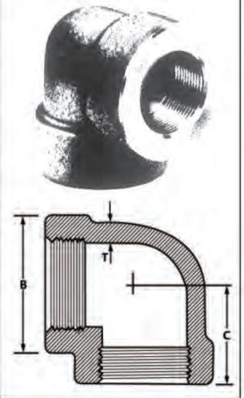
90° elbows
