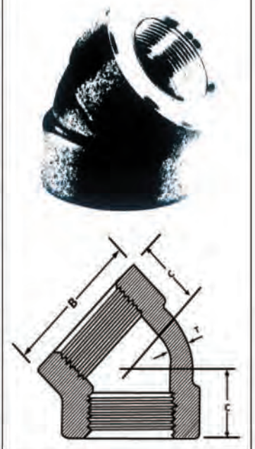
45° elbows
